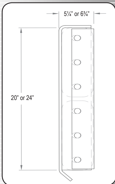
Dock Defender™
