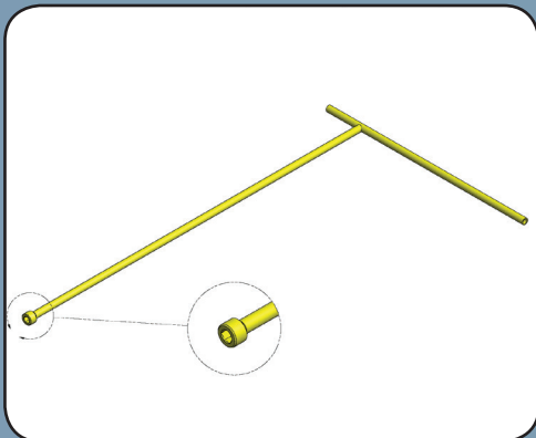
Figure 1: Power Release Tool drawing highlighting bolt head fitting
