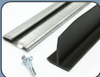
Figure 4: PVC with aluminum channel
