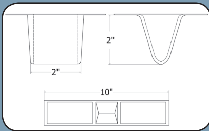
Figure 1: Door Sprag schematics
