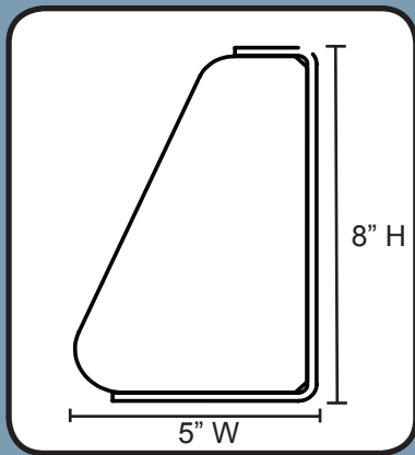
Figure 2: Fork Sentry Dimensions
