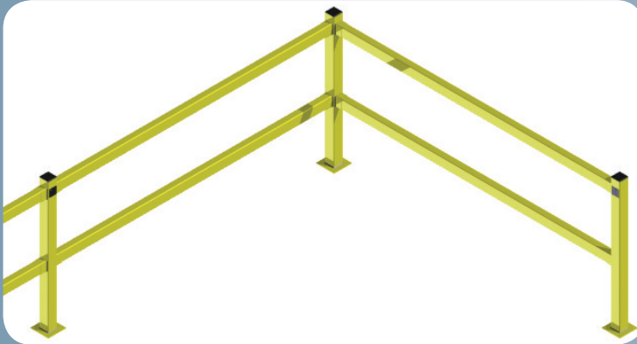
Figure 1: Double-rail with end post, corner post and continuous post.
