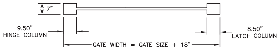
Gate Layout (Top View)
